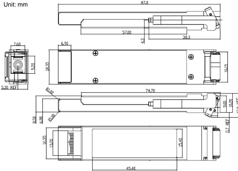
Figure 7 Package Outline
