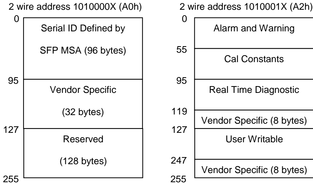
Fig 2 EEPROM Information
