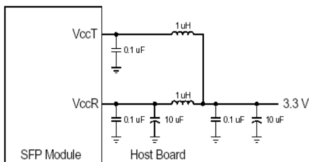
Figure3. Host Board Supply Filtering Circuit
