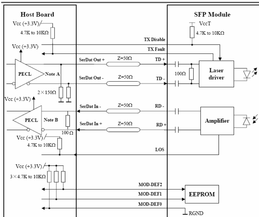
Figure4. Application Circuits
