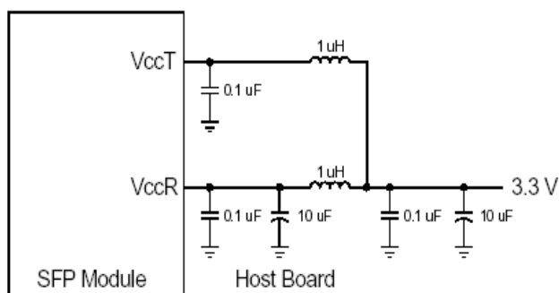
Figure3. Host Board Supply Filtering Circuit
