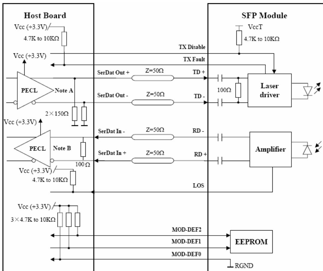
Figure4. Application Circuits
