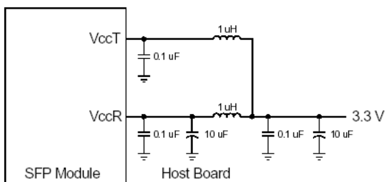
Figure3. Host Board Supply Filtering Circuit
