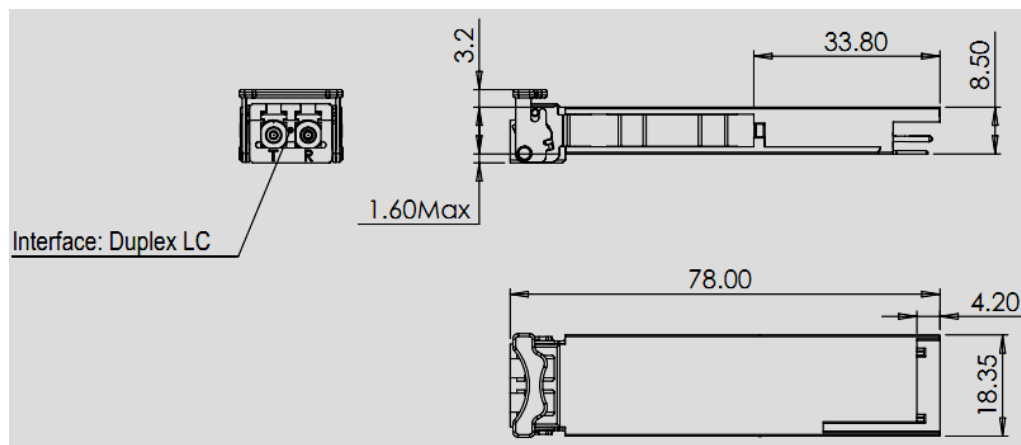
Figure 4. Mechanical Outline
