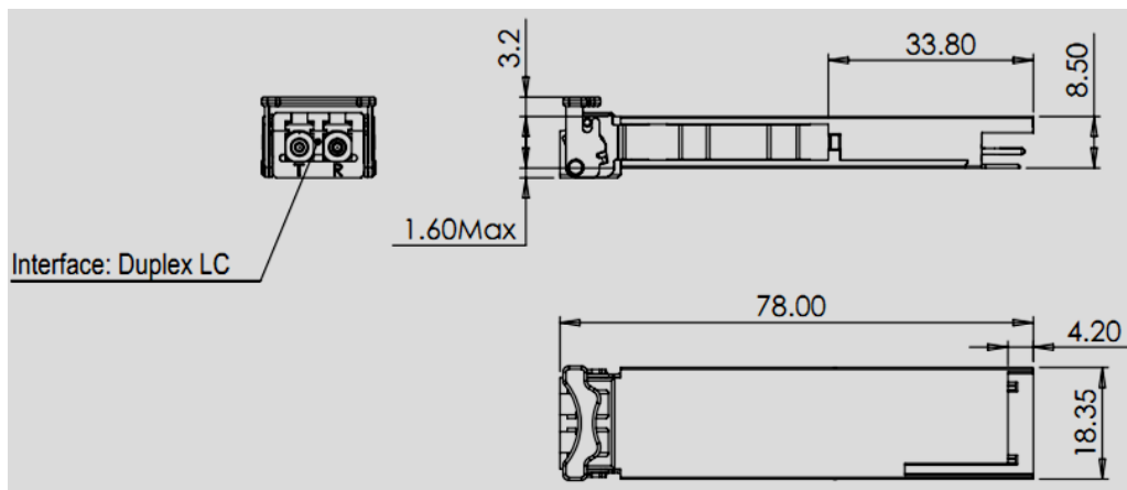
Figure 4. Mechanical Outline
