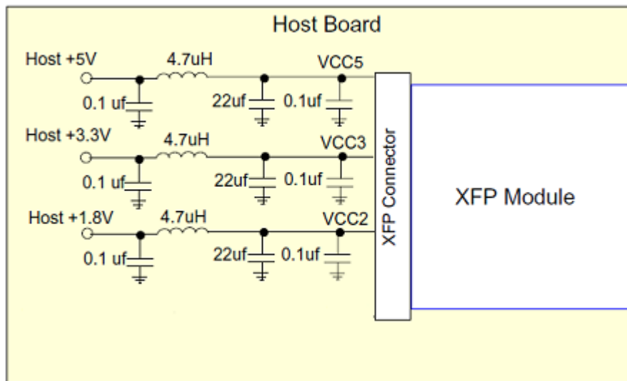
Figure 1, Recommended Host Board Power Supply Circuit
