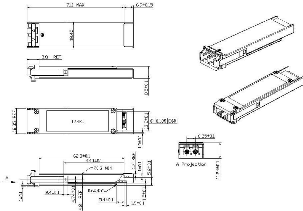
Figure 4, Mechanical Diagram of XFP
